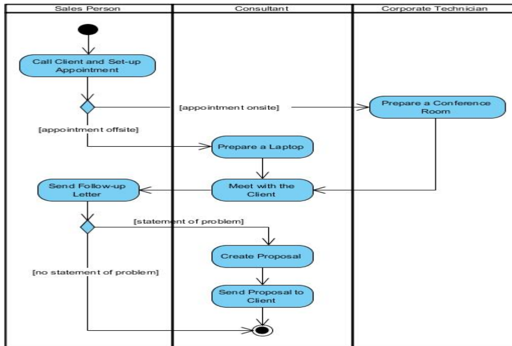
Figure 7: Activity diagram formalism
