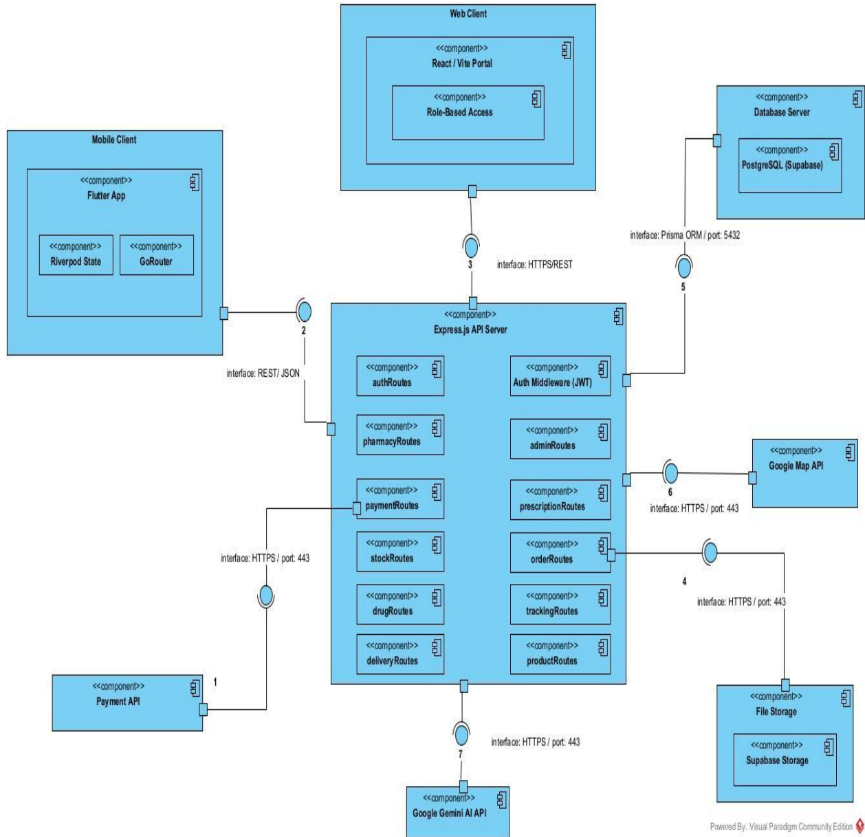
Figure 31 : component diagram
