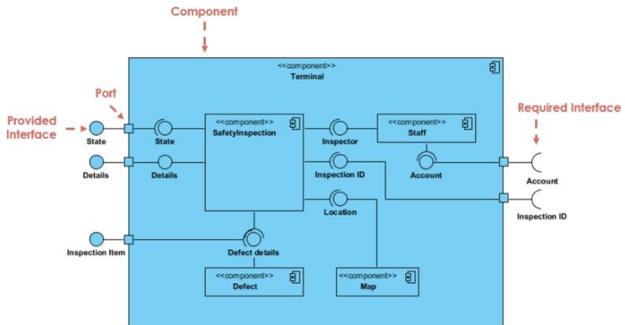
Figure 30 : Component diagram formalism
