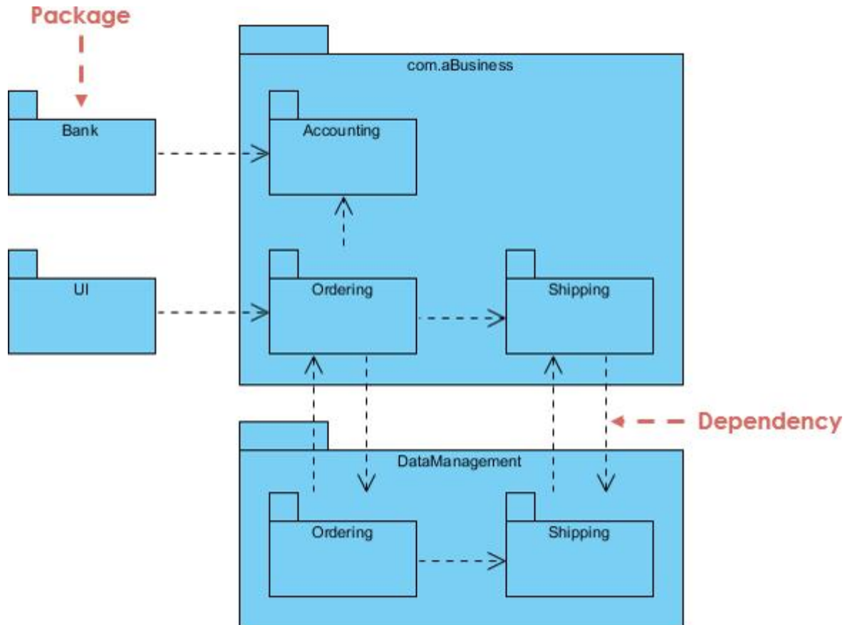
Figure 28 : Package diagram formalism
